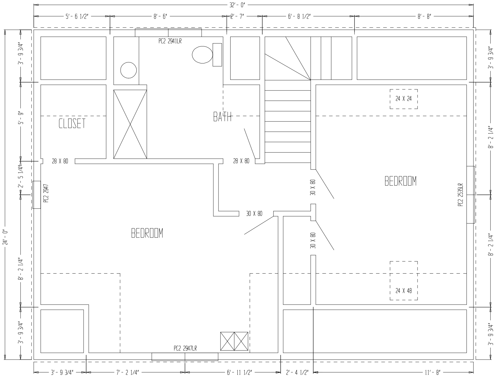
UPPER LEVEL PLAN, FARNUM 3/4/01
